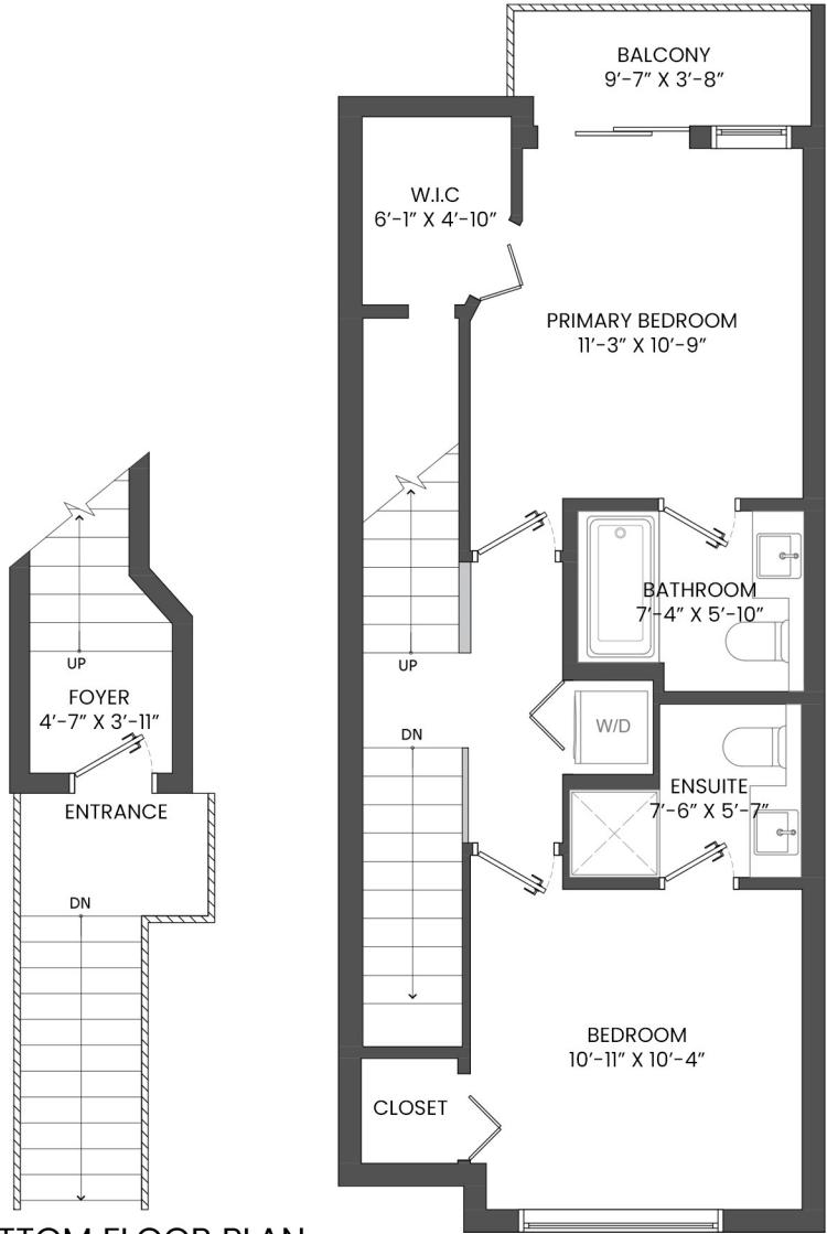
LOWER FLOOR PLAN Ceiling Height: 8'-0"
