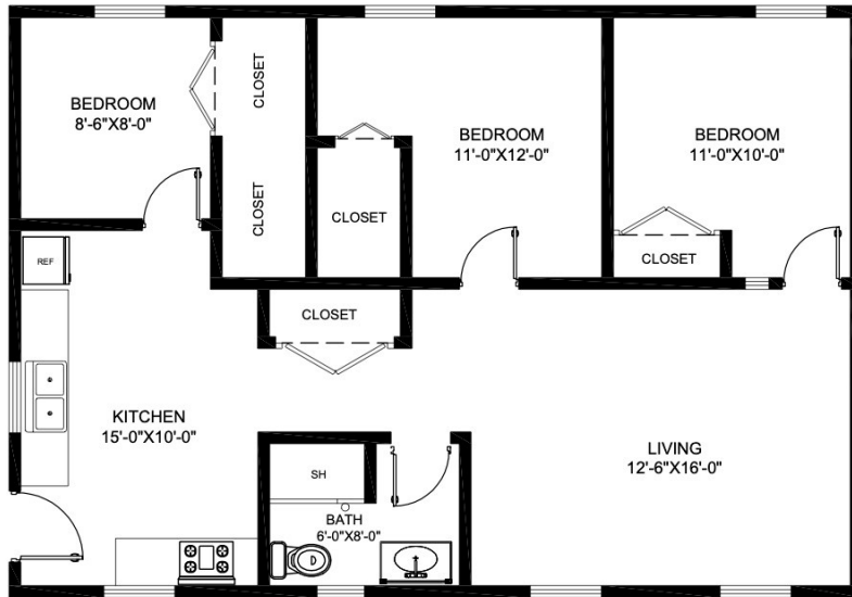
BASEMENT PLAN
