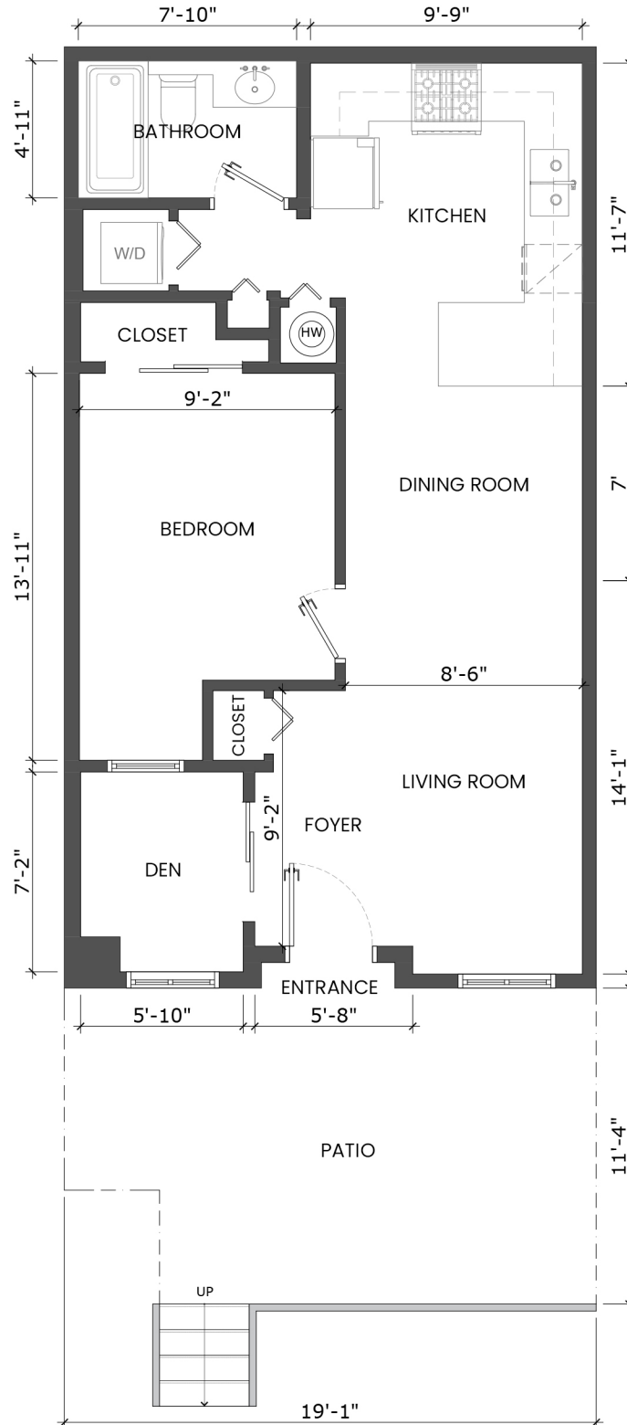
MAIN FLOOR PLAN Ceiling Height: 8'-0"
