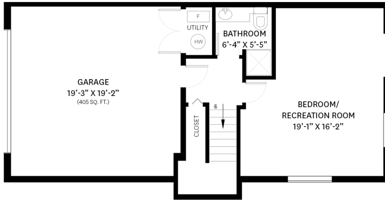
LOWER FLOOR PLAN Ceiling Height: 8'-0"
