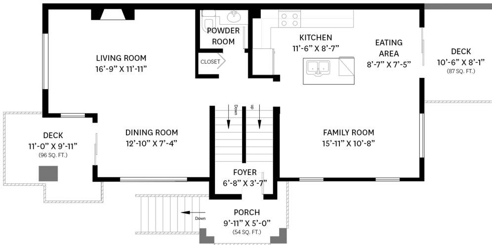
MAIN FLOOR PLAN Ceiling Height: 8'-11"
