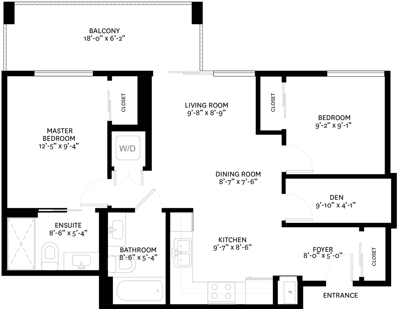
MAIN FLOOR PLAN Ceiling Height: 8'-11"
