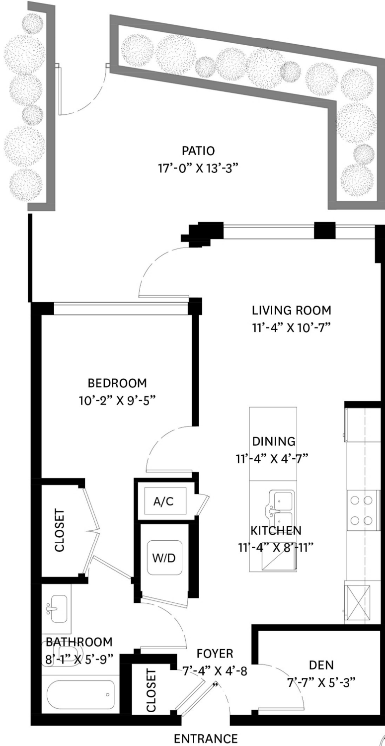
MAIN FLOOR PLAN Ceiling Height: 8'-10"
