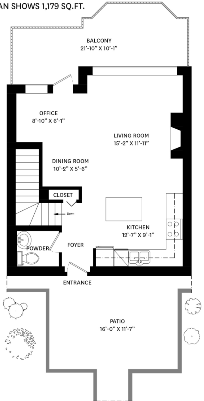
MAIN FLOOR PLAN Ceiling Height: 9'-4"
