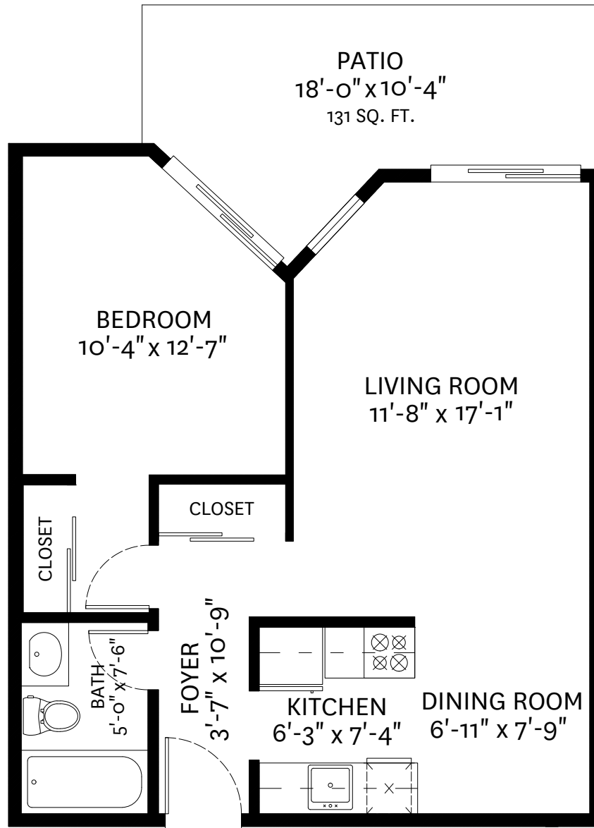
FLOOR PLAN Ceiling Height: 8'-0"
