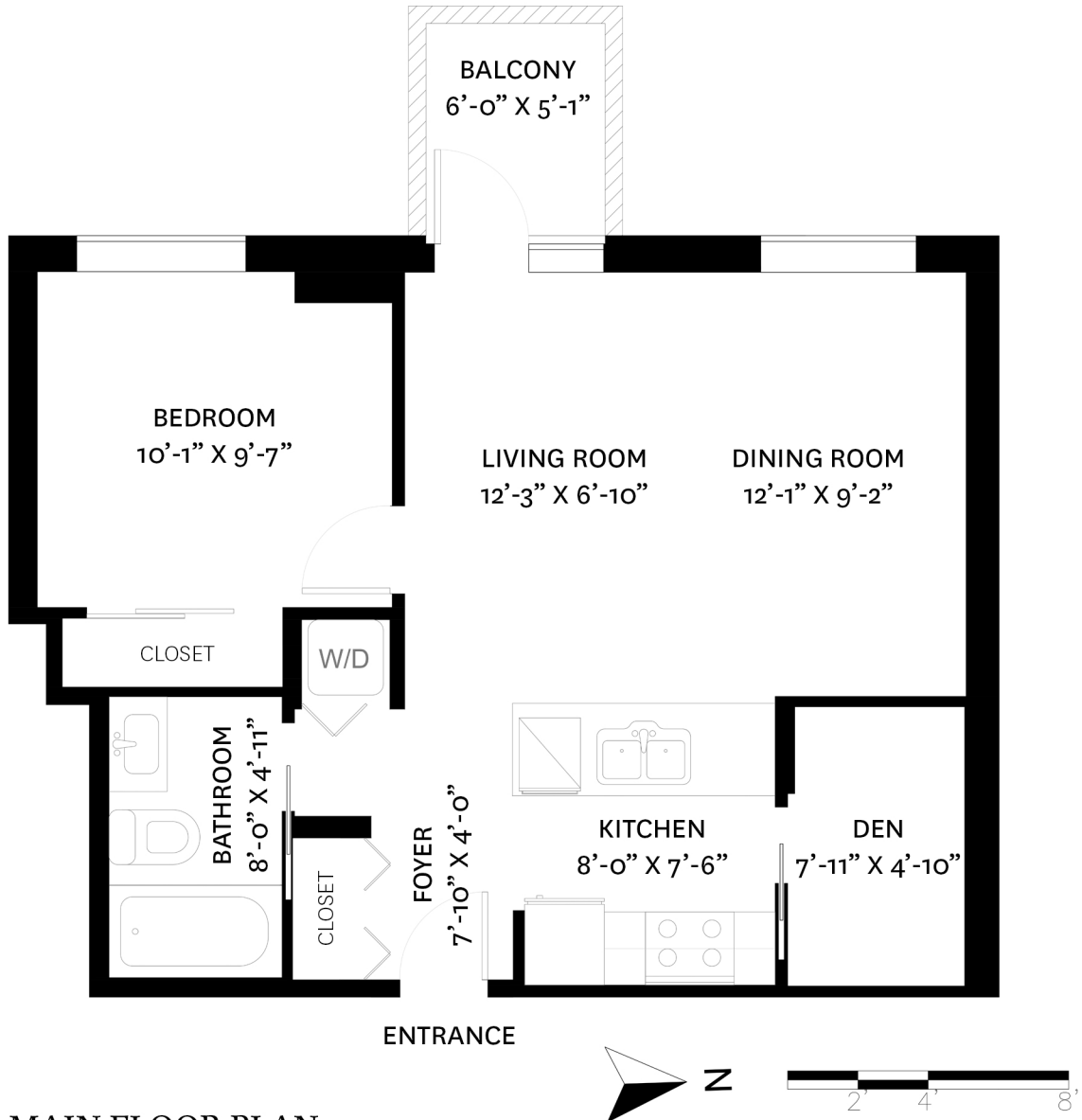
MAIN FLOOR PLAN Ceiling Height: 8'-2"
